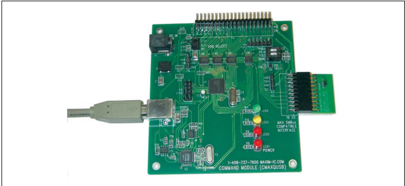
Figure 2. CMAXQUSB with DS28CM00 Evaluation Board
