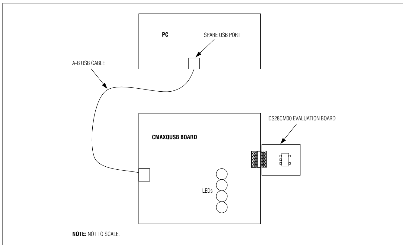
Figure 1. Typical Setup
